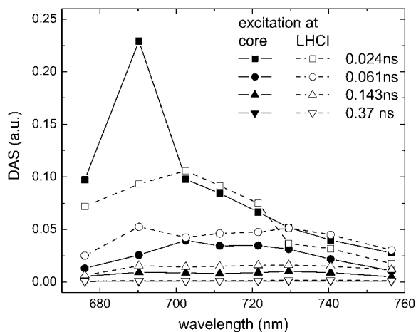
FIGURE 7 Decay associated spectra of PSI-LHCI in solution at 287 K, after (hypothetical) excitation of only core or only LHCI pigments (dashed lines). DAS were calculated from linear combinations of the DAS in Fig. 3, with 65% core excitation at 410 nm, and 30% at 475 nm. See text for more details. In Fig. S12 (Data S1), the three slow DAS are presented after scaling to equal area.
