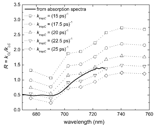
FIGURE 8 Ratio R = k_{CL}/k_{LC} calculated from the ratio between the absorption spectra of LHCI and core, and calculated from the average lifetime after selective excitation of core pigments ( \bar{\tau}^C ) and various rates of trapping from the core ( k_{\text{trapC}} ), using R = k_{\text{trapC}} \times \bar{\tau}^C - 1 (see Discussion and Appendix A). R calculated by these two methods coincides rather well for k_{\text{trapC}} = (22.5 \pm 2.5 \text{ ps})^{-1} . This number was not affected by fixing the fastest lifetime to values ranging from 15 to 30 ps and reoptimizing the fit of the fluorescence decay traces.
