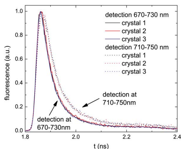
FIGURE 2 Normalized sums of fluorescence decay curves of three different PSI-LHCI crystals measured at room temperature with FLIM. Excitation was at 860 nm, detection at 670–730 nm (solid lines) and 710–750 nm (dotted lines).
